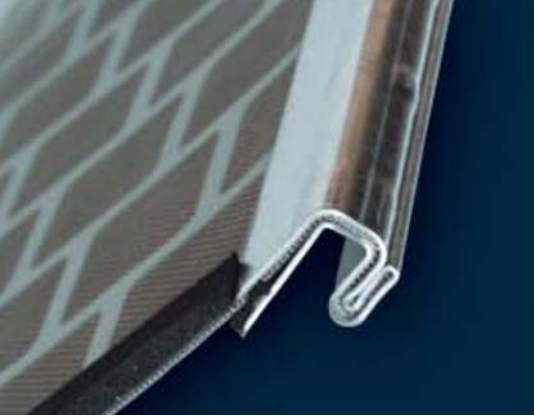
Hook strip formats of NEXTweave Shaker Screens for all major brands of Shale Shaker.
