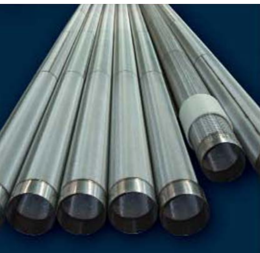
Sand Control Screens used during well completions made from Diffusion bonded Filtration Media „POROSTAR“
